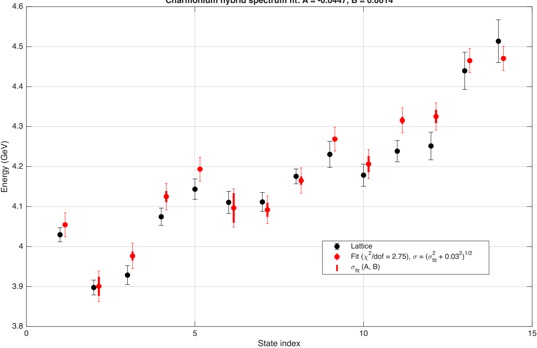
Charmonium hybrid spectrum fit: A = -0.0447, B = 0.0014
